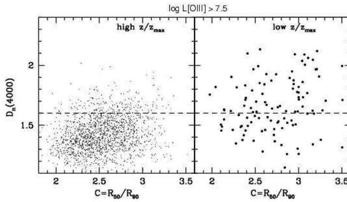
Figure 20: AGN with [OIII] luminosities greater than 10^{7.5} L_\odot are plotted in the D_n(4000)/C plane. In the left panel we show objects with z/z_{max} > 0.8 . In the right panel, we show objects with z/z_{max} < 0.3 .
